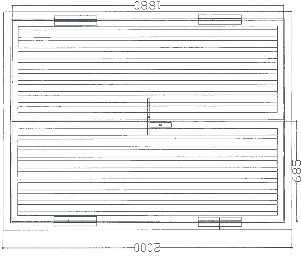
Front Elevation for DAS Cover
